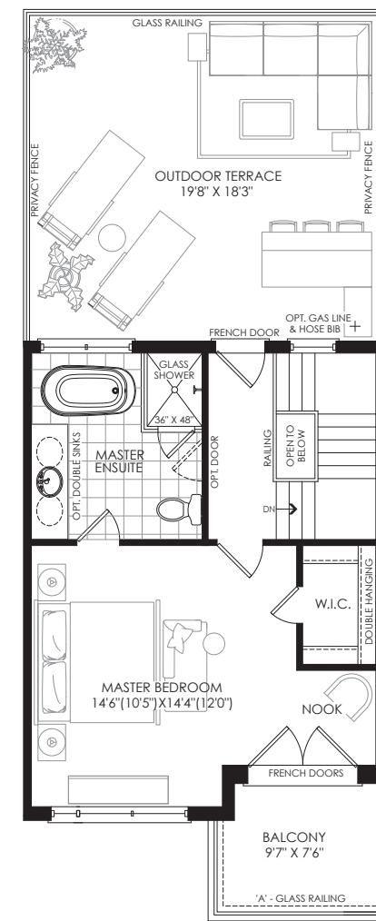
THIRD FLOOR PLAN ELEV. 'A', 'B'
